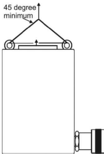
Figure 1 – Hoisting Cylinder
