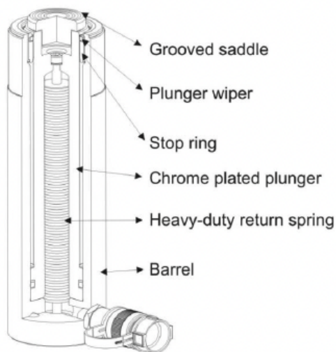
Figure 2 – RG Series Sectional Drawing
