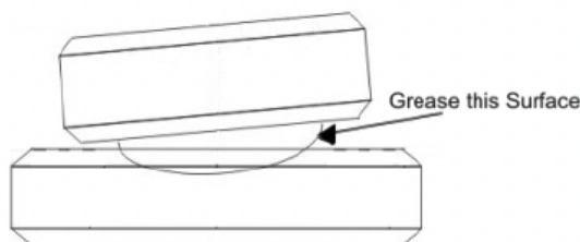
Figure 3 – Tilt Saddle.
